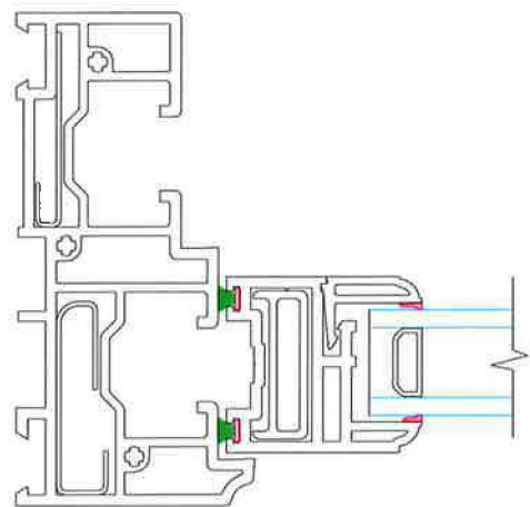
Frame Detail (B-B) Scale 1:2
