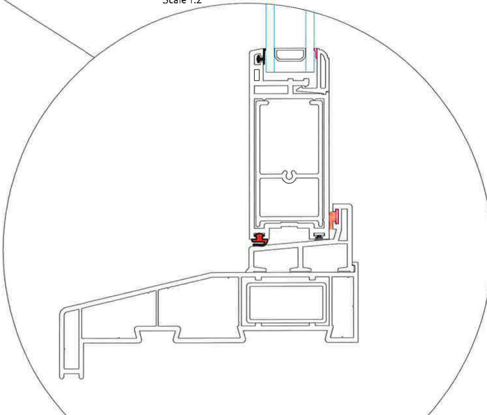
Window Details Scale 1:2
