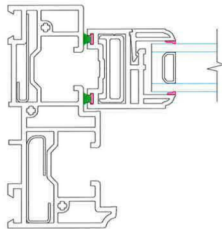
Frame Detail (C-C) Scale 1:2
