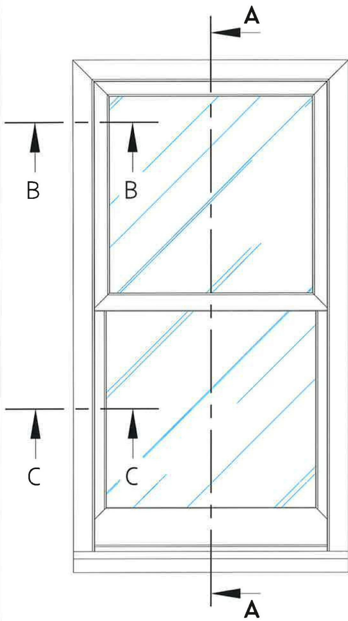
Sliding Sash Elevation Scale 1:10
