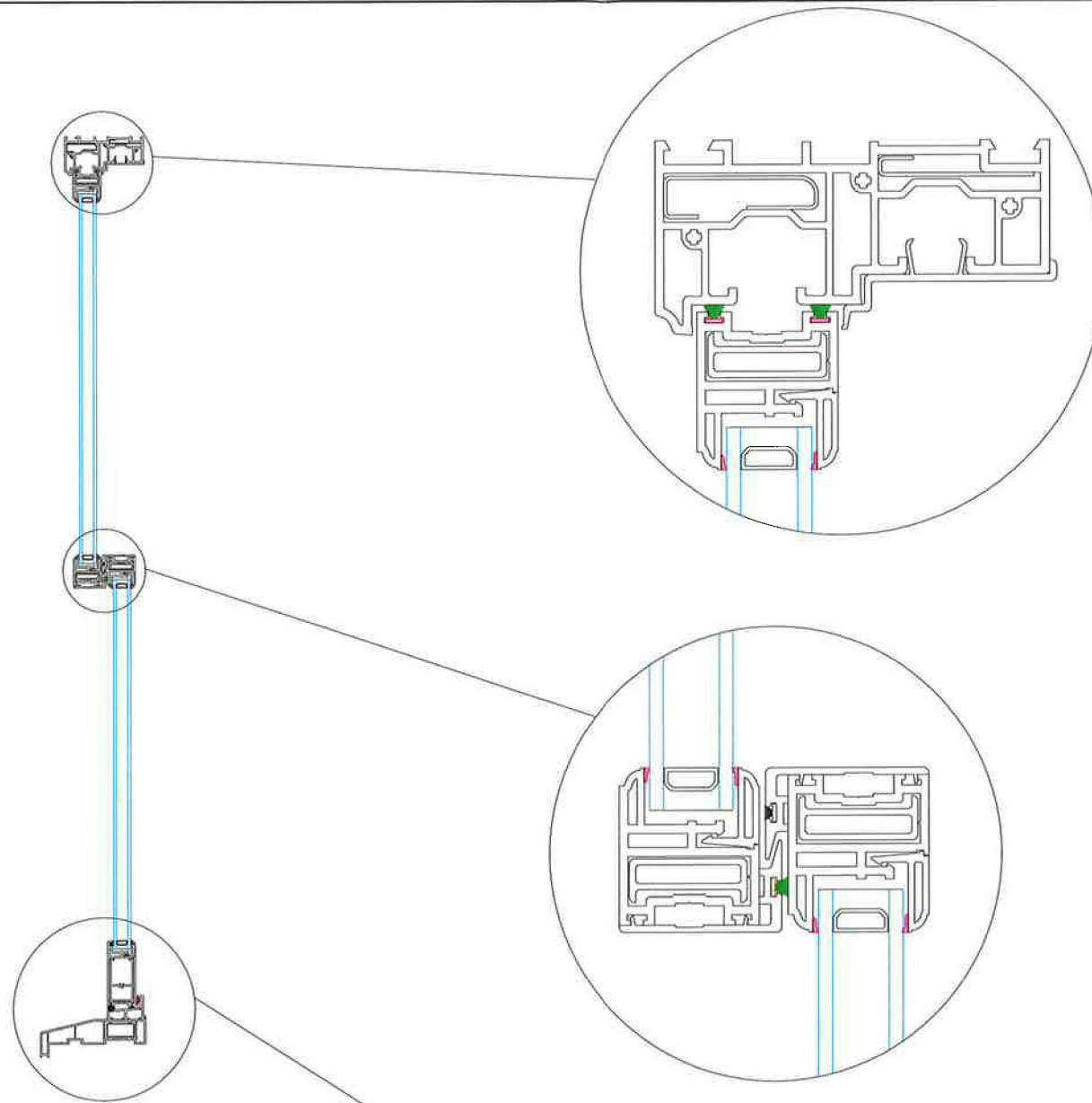
Window Details Scale 1:2
