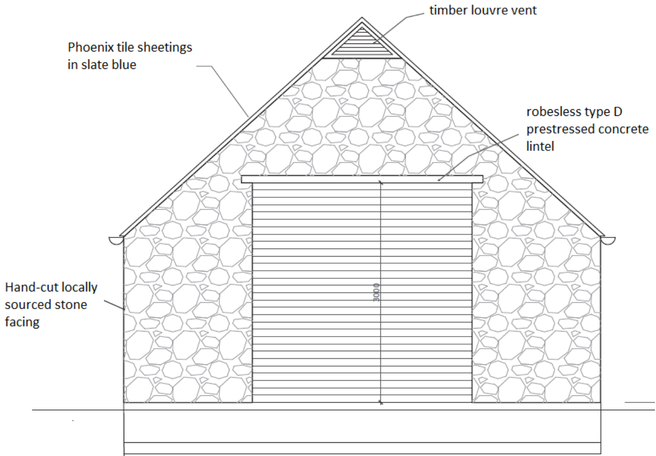
Front Elevation
