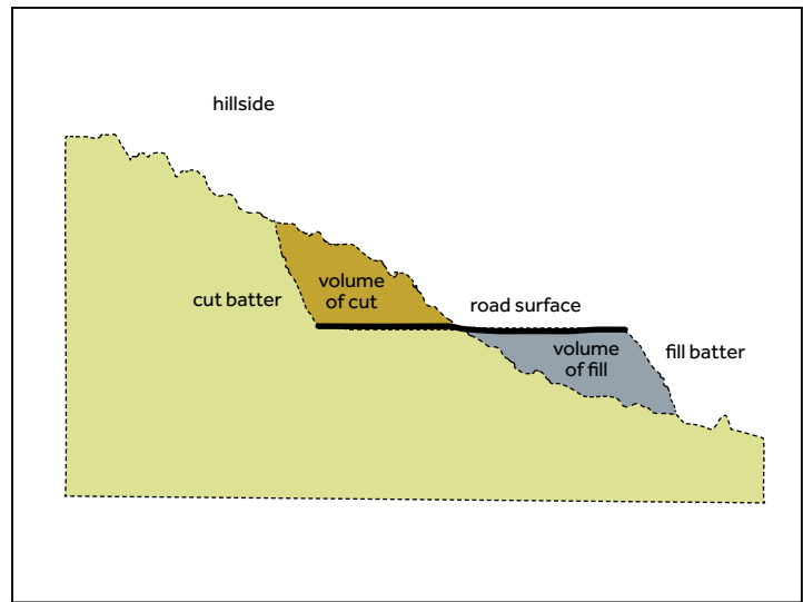
Figure 5 Diagram of cut and fill batters
