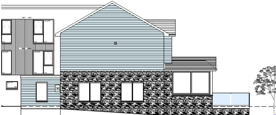
West Elevation as Proposed showing front extension and rear extension, glass balustrade and new cladding to first floor.
